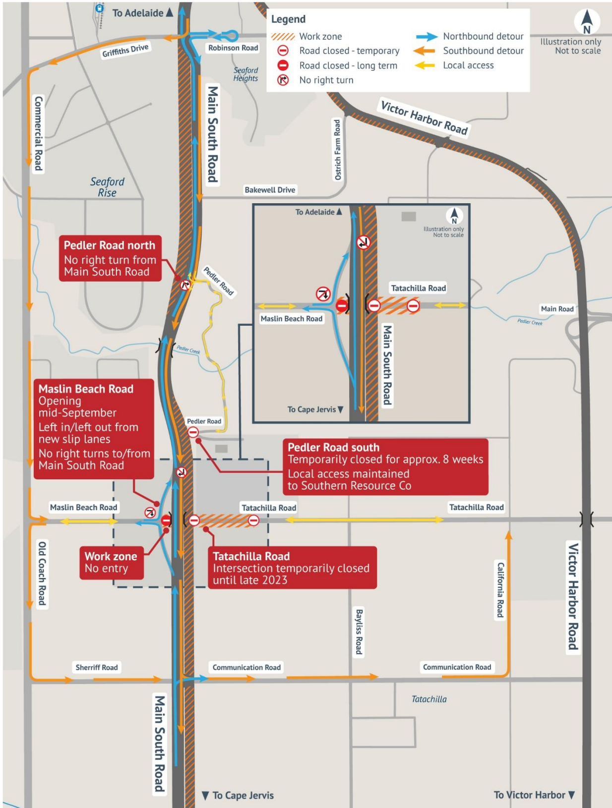
Map 2 – Tatachilla Overpass Post Traffic Switch
